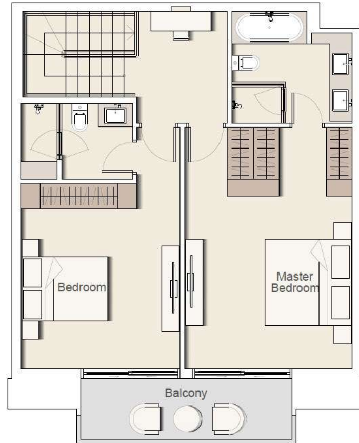
Podium Level
